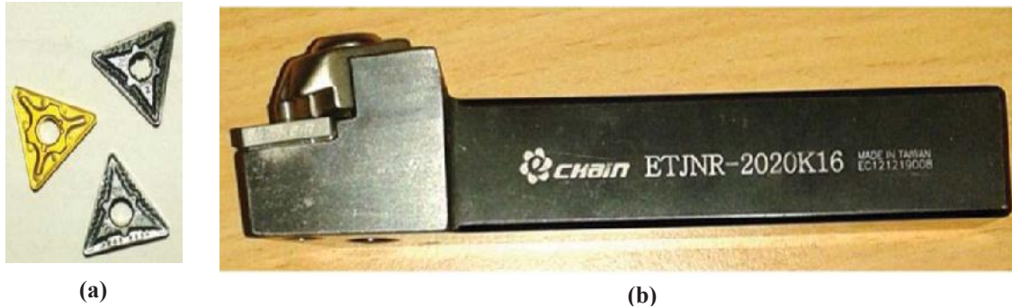
FIGURE 1. Cutting tools used in the study, (a) Carbide insert cutting tool, (b) Cutting tool handle
